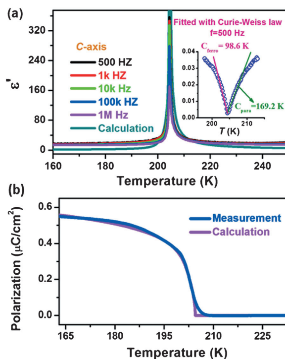
Figure 3. Dielectric and polar response for the transition at 205 K. a) The temperature dependence of the real part of the complex dielectric constant in the c -direction. Inset: Plot of 1/\epsilon' versus temperature. b) The temperature dependence of the spontaneous electric polarization P_s calculated by integrating the pyroelectric current upon cooling.
